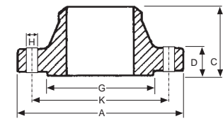
WELDING NECK (WN)
