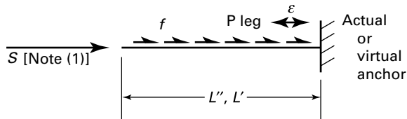
Figure VII-3.3.2-4 Element Category D, Straight Pipe
